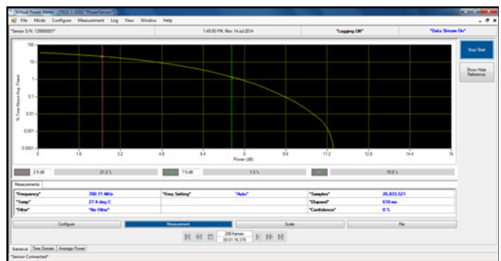
Figure 4 - Statistical Power Display
