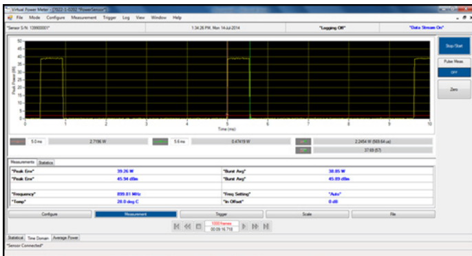
Figure 3 - Time Domain Mode
