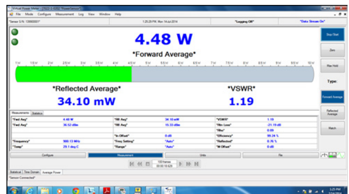
Figure 2- Conventional Power Measurement Mode
