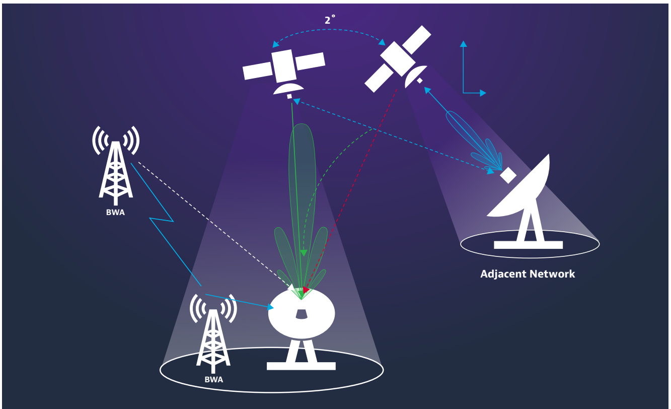
Figure 3: Interaction between satellite earth stations and broadband wireless nodes
