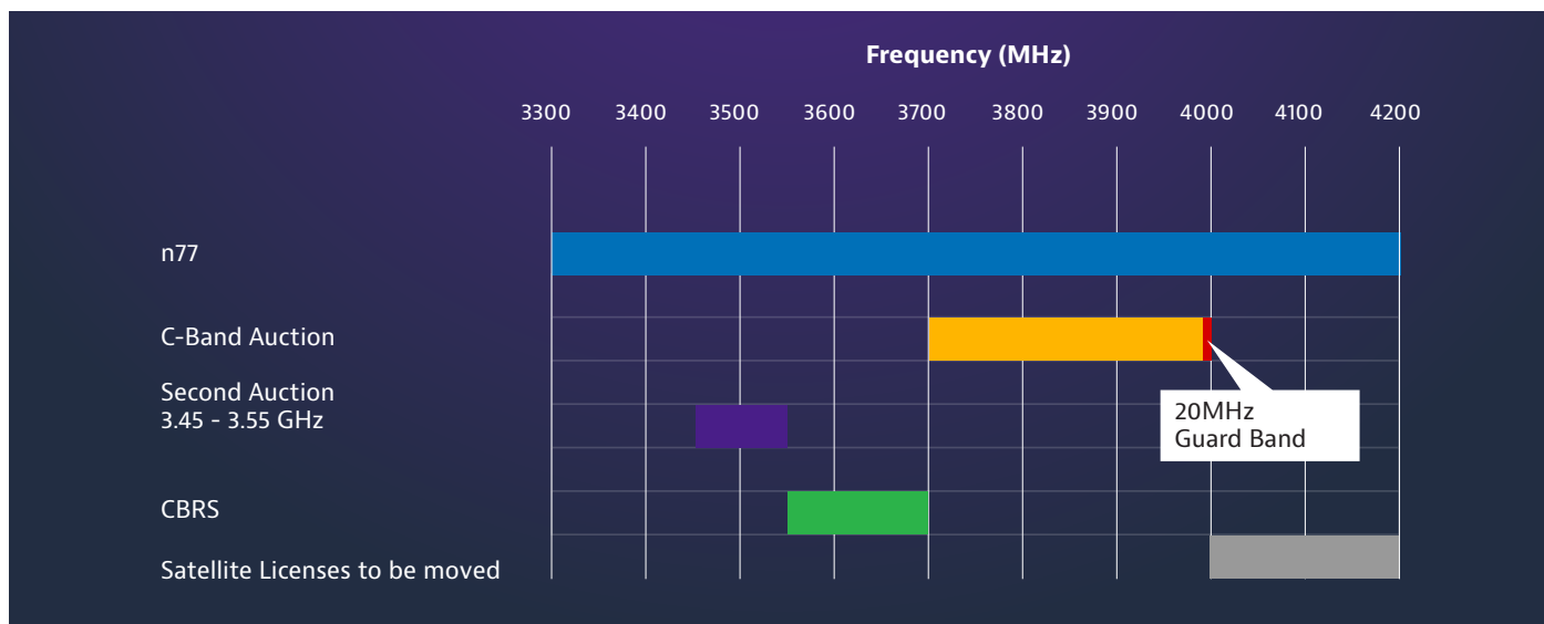
Figure 1: C-band spectrum in the US
