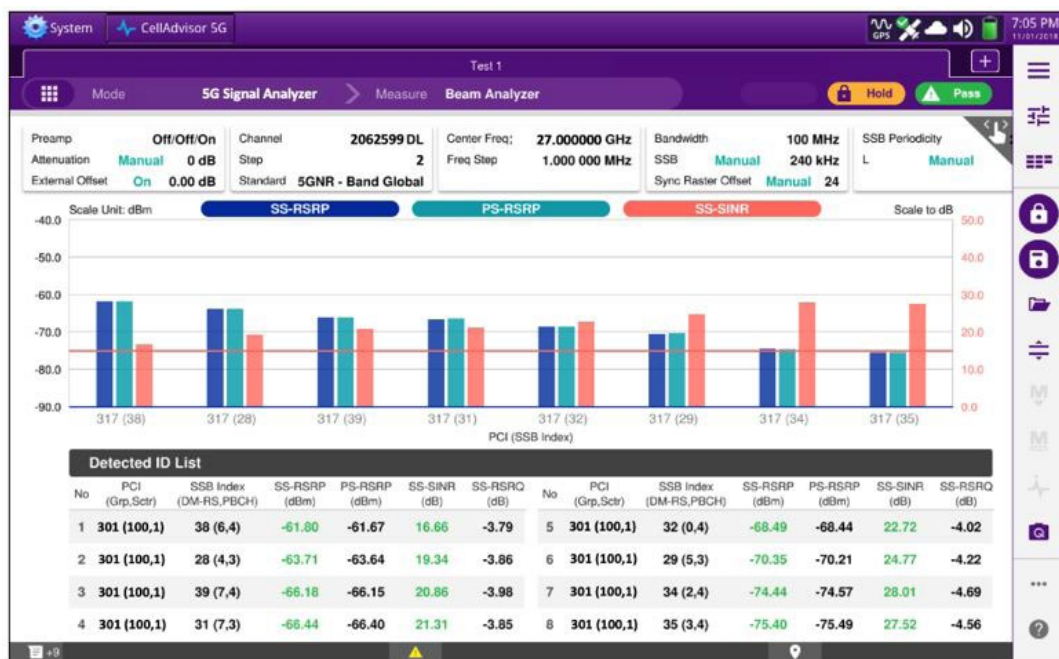
Figure 10: CellAdvisor 5G Beam Analyzer (8 strongest beams)
