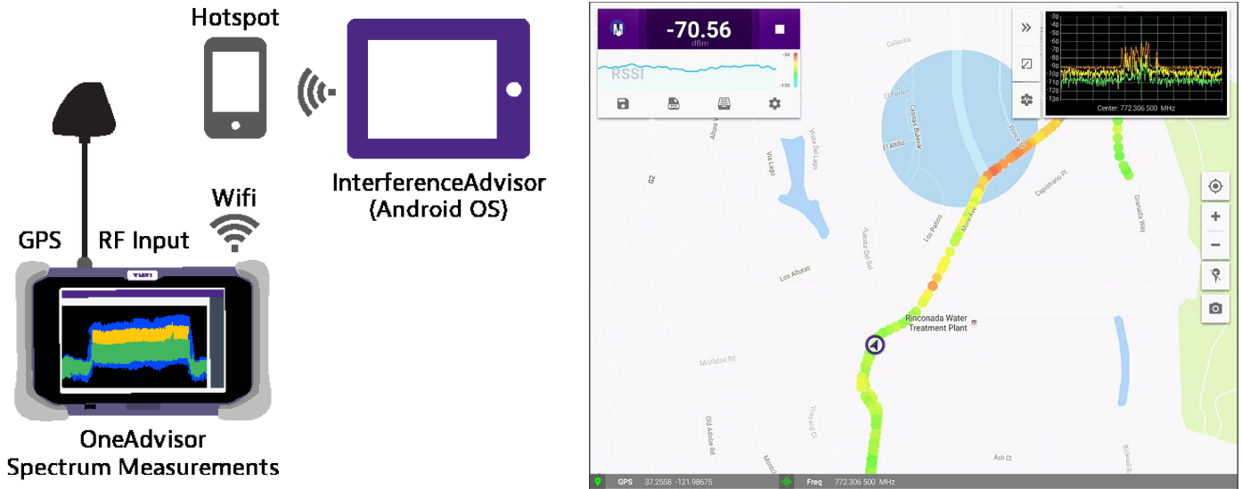
Figure 2: Spectrum Analyzer and InterferenceAdvisor solution overcome RF interference challenges
