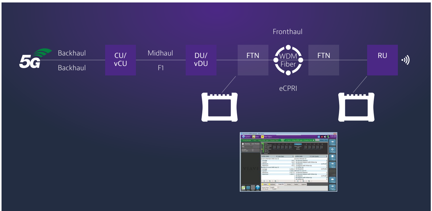
Figure 6: Example of 5G fronthaul RU connectivity and delay test
