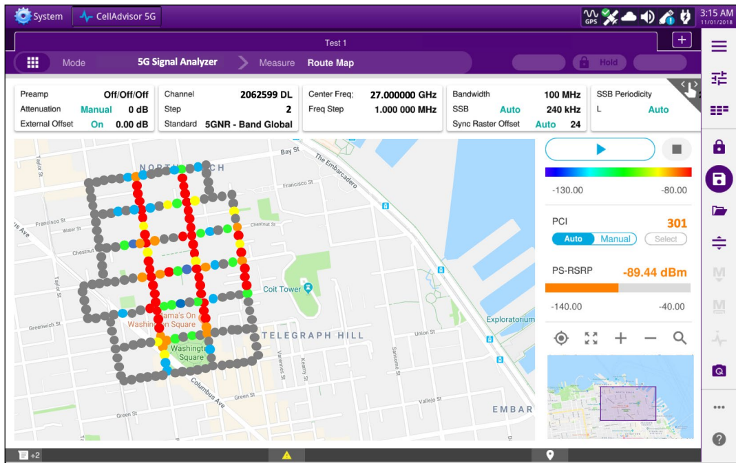
Figure 11: CellAdvisor 5G coverage map analysis
