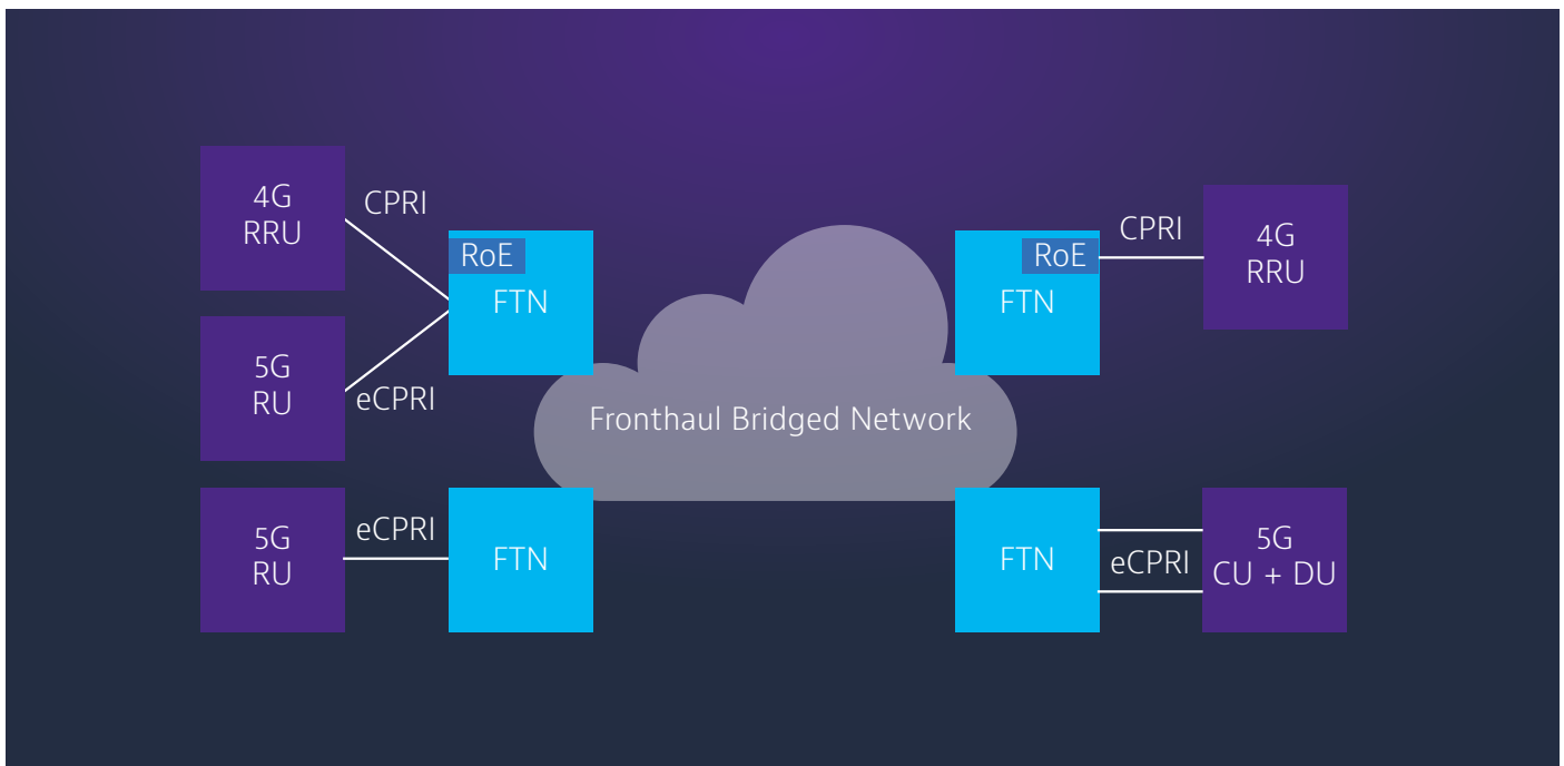
Figure 5: FTN Network architecture
