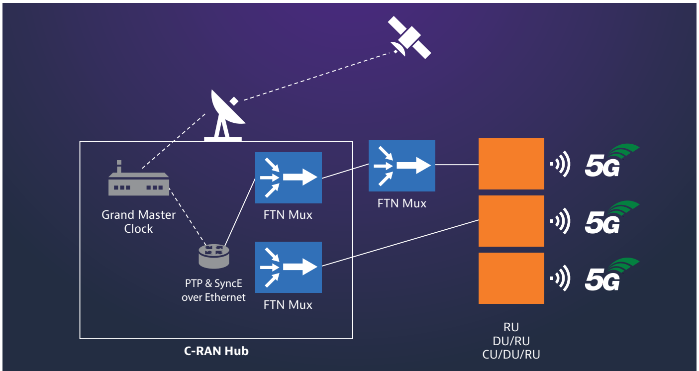
Figure 7: Timing distributed over 5G-NR network
