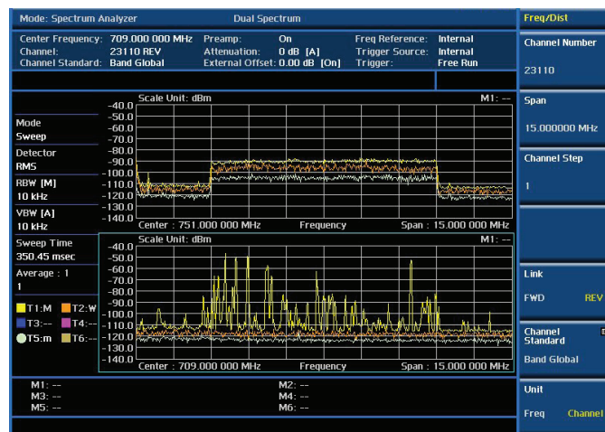
RF test — Dual Spectrum
