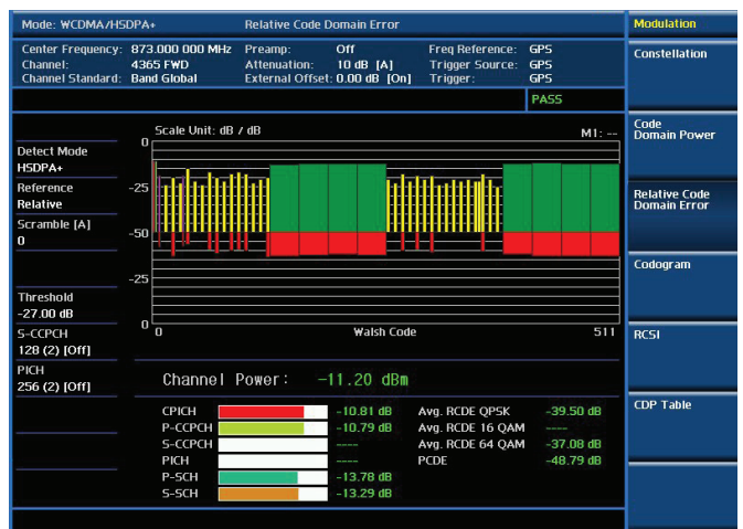
Modulation analysis — Relative Code Domain Error
