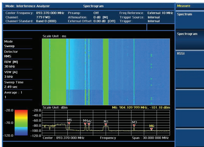
Interference analysis test — Spectrogram
