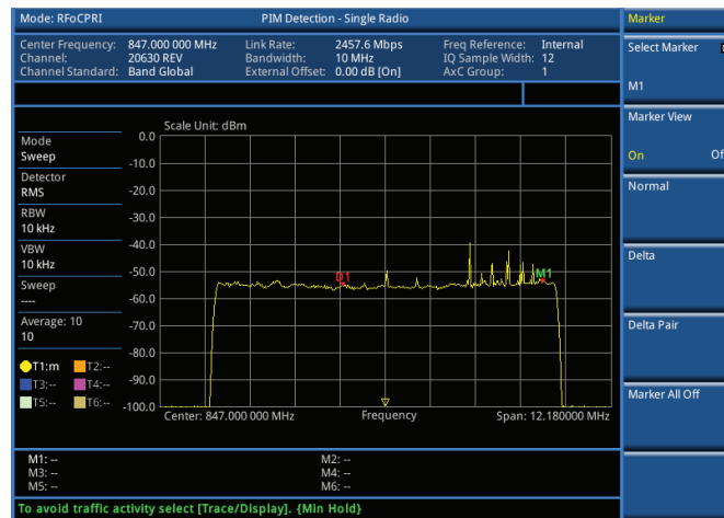
RFoCPRI — Detection - Single Radio
