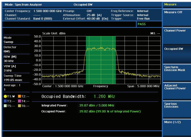
RF analysis — Occupied Bandwidth
