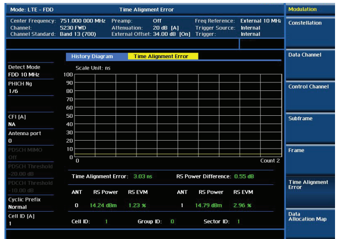
Modulation analysis — Time Alignment Error
