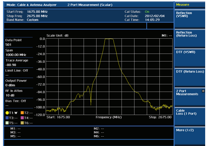
2-Port Measurement (Scalar) function
