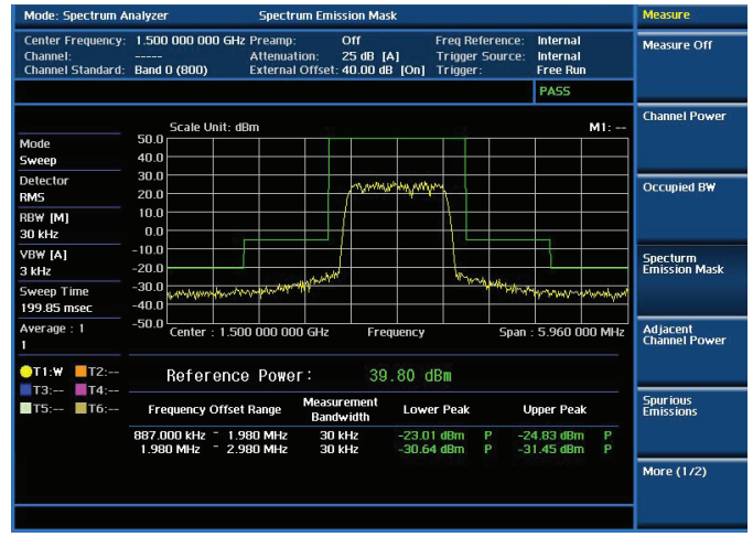
RF test — Spectrum Emission Mask
