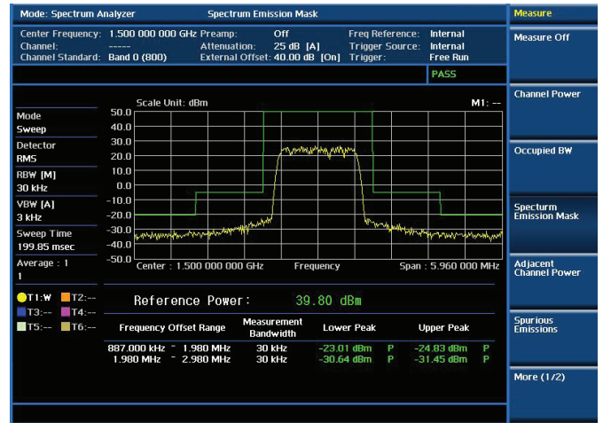
RF analysis — Spectrum Emission Mask
