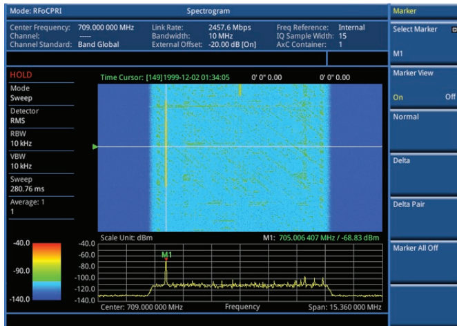
RFoCPRI — Spectrogram
