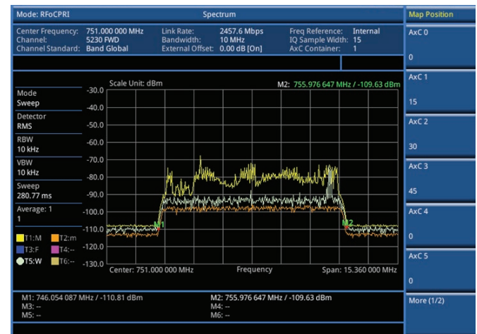
RFoCPRI — Spectrum
