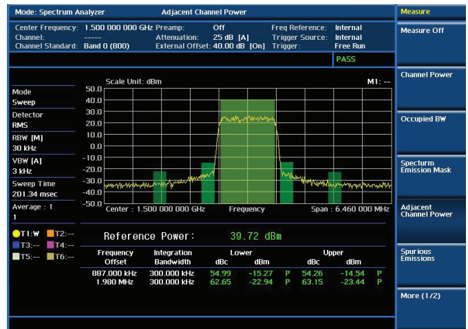
RF analysis — Adjacent Channel Power
