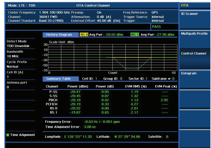
OTA analysis — Control Channels
