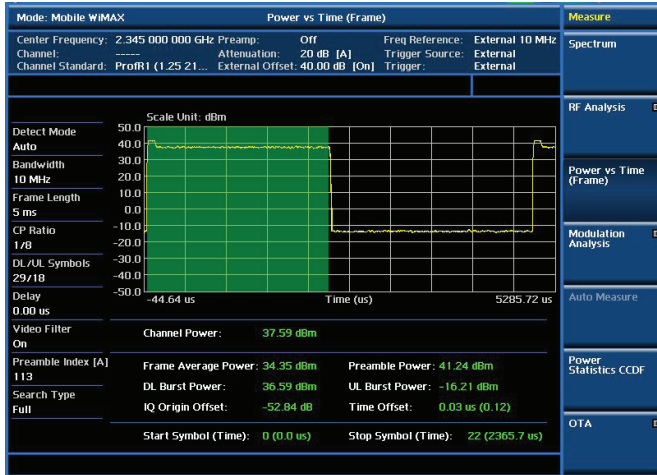
Modulation analysis — Power vs. Time (Frame)
