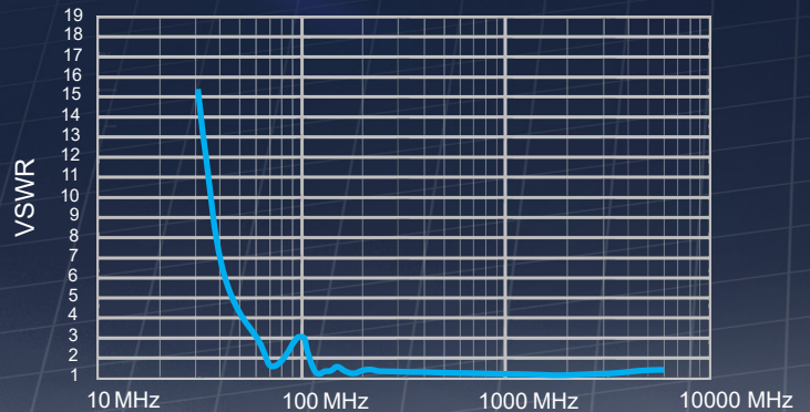
BL-01 - VSWR
